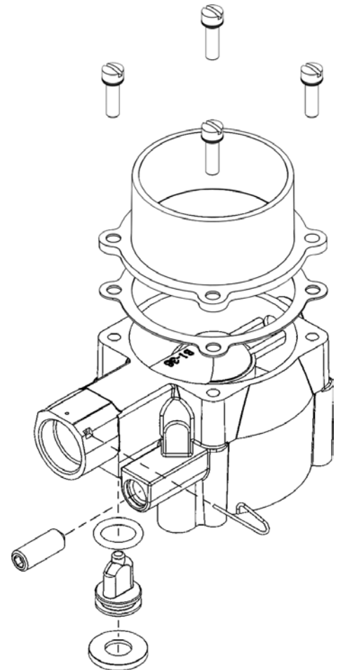
Right: New Model 55M-500 Body with the new Idle Screw and Power Valve, now adjusted from the bottom (shown with air horn and hardware).
